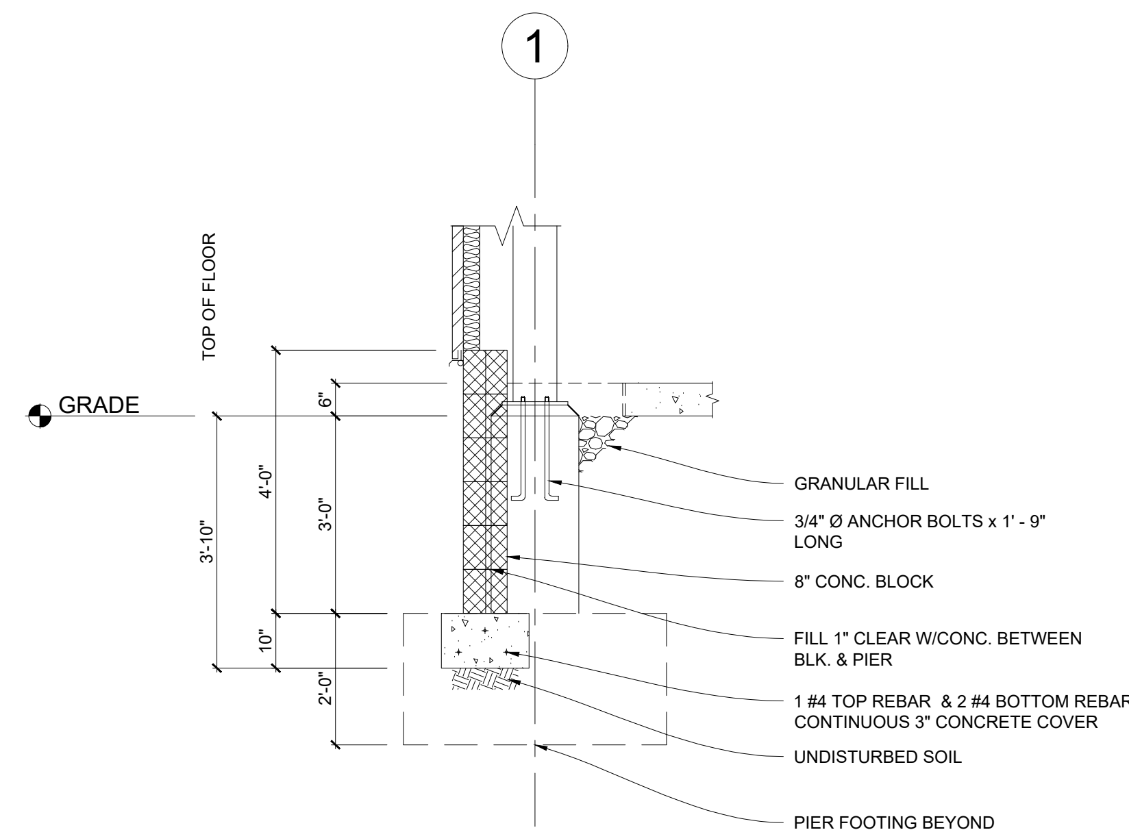
7 SECTION C1 DETAIL SCALE: 1/2" = 1' - 0"
