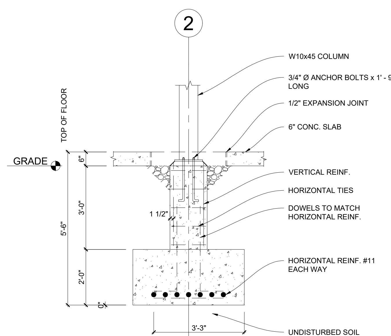
6 SECTION B2 DETAIL SCALE: 1/2" = 1' - 0"
