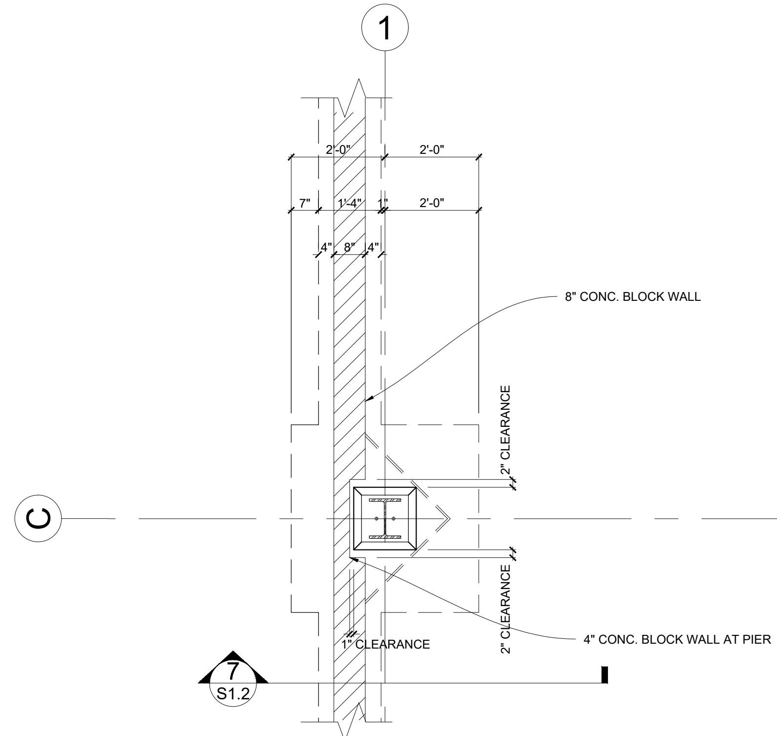
4 FOUNDATION C1 DETAIL SCALE: 1/2" = 1' - 0"
