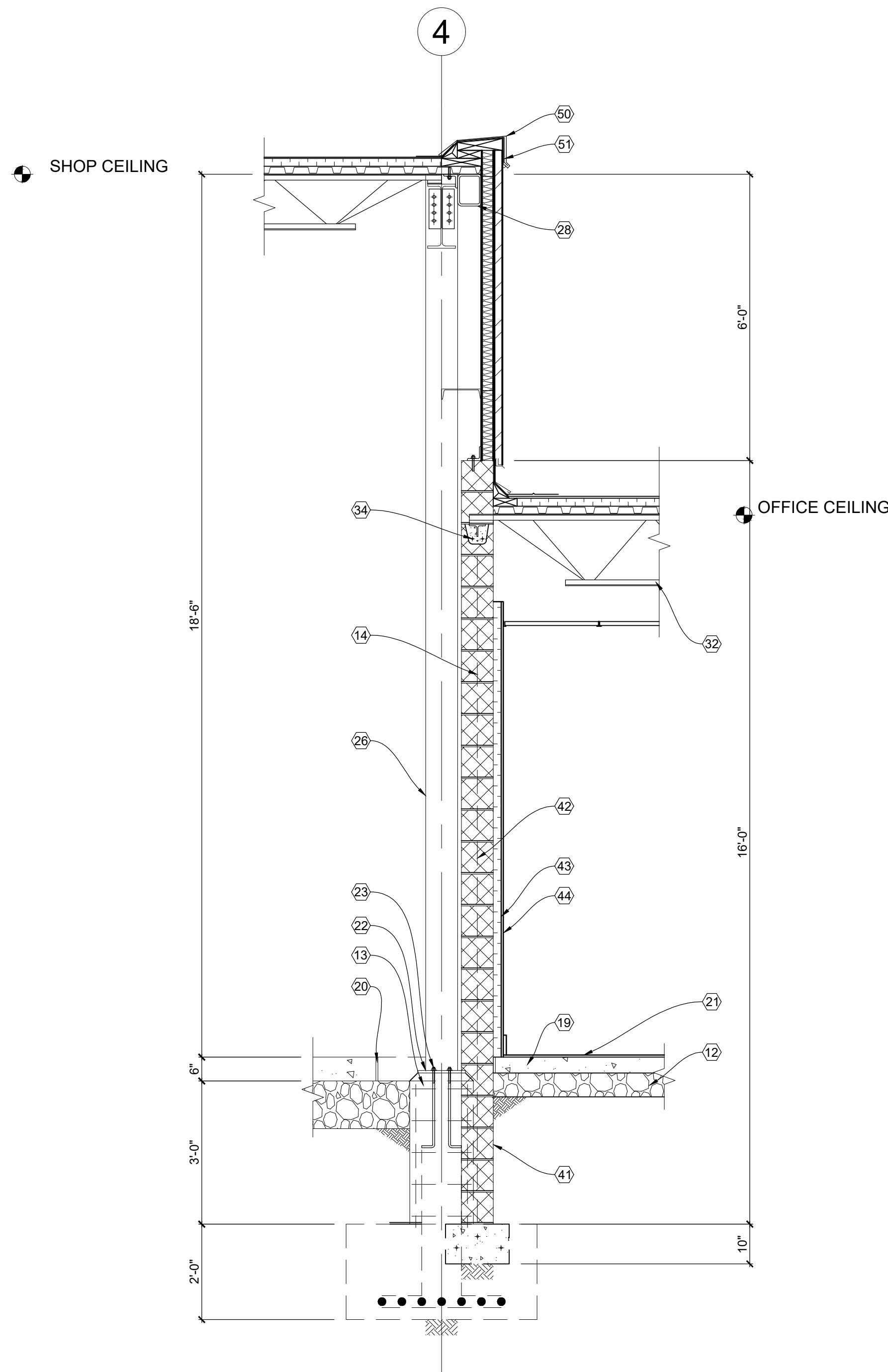
1 WALL SECTIONS SCALE: 1/2" = 1'-0"
